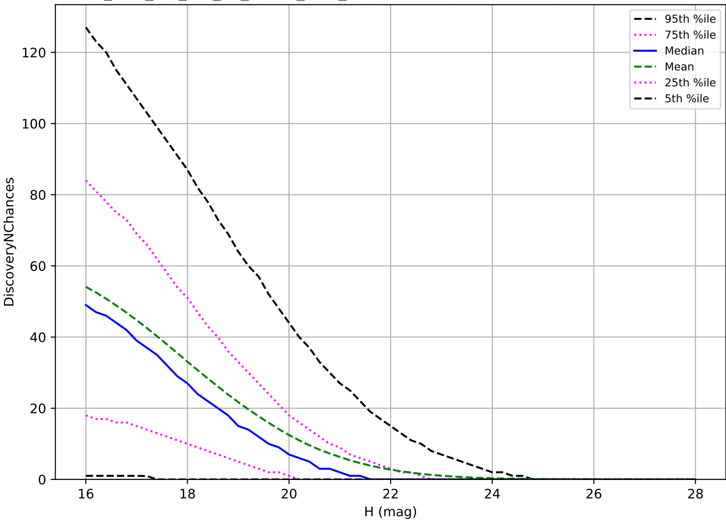
too_elab_2yr_r32_d2_ugrizy_v3.4_10yrs: PHA 3 pairs in 15 nights detection loss
