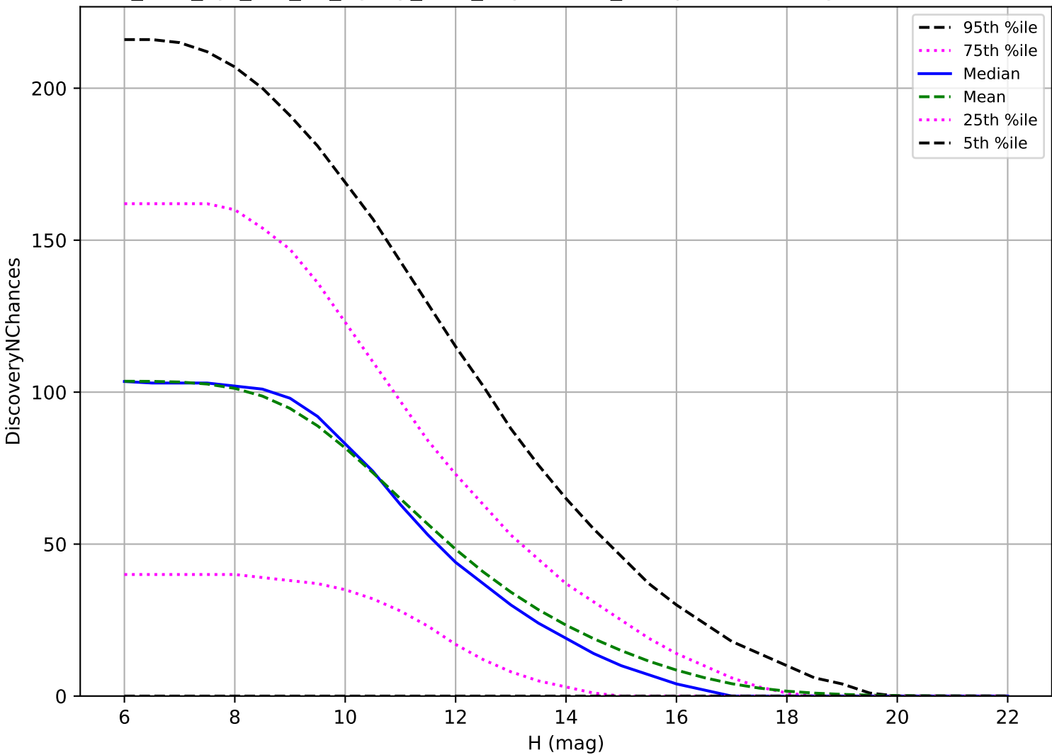
too_elab_2yr_r32_d2_ugrizy_v3.4_10yrs: OCC_r5 3 pairs in 15 nights detection loss
