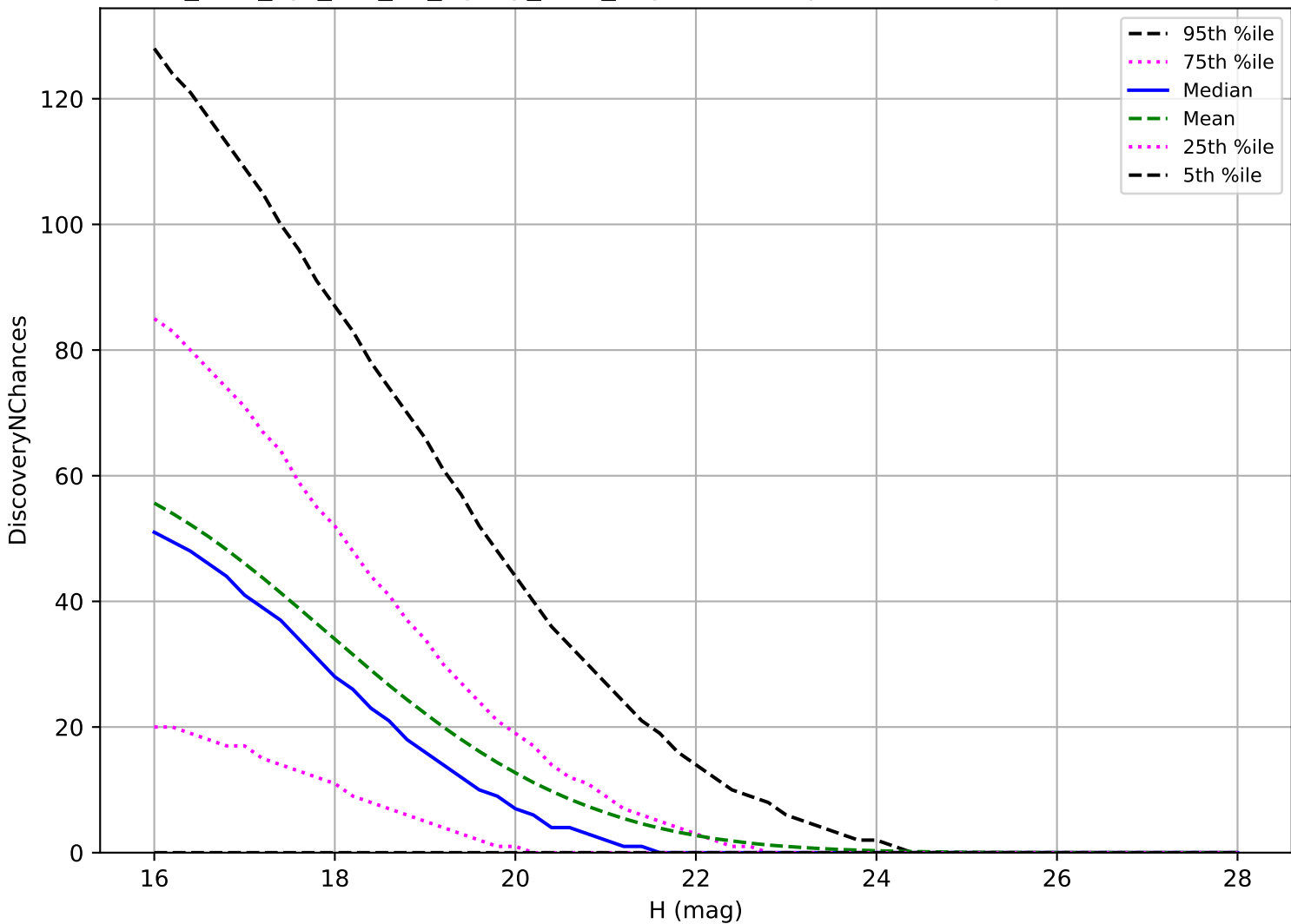
too_elab_2yr_r32_d2_ugrizy_v3.4_10yrs: NEO 3 pairs in 15 nights detection loss
