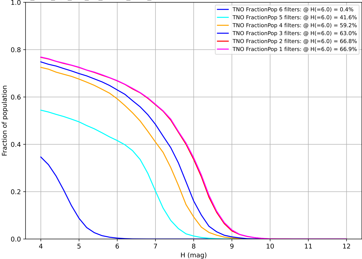
too_elab_2yr_r32_d2_ugrizy_v3.4_10yrs: Fraction of population with colors in X filters TNO
