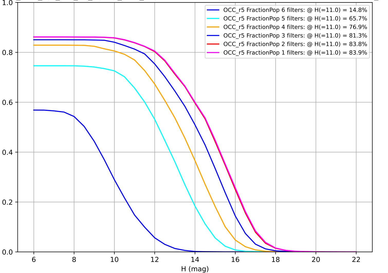
too_elab_2yr_r32_d2_ugrizy_v3.4_10yrs: Fraction of population with colors in X filters OCC_r5
