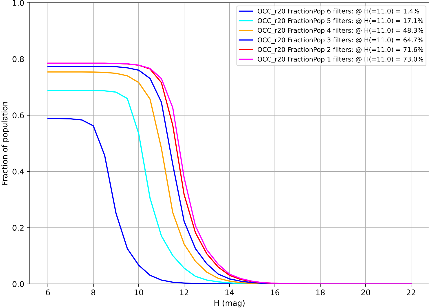
too_elab_2yr_r32_d2_ugrizy_v3.4_10yrs: Fraction of population with colors in X filters OCC_r20
