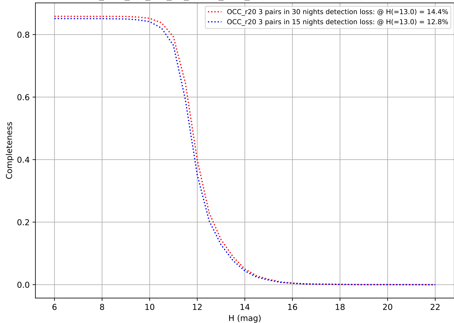
too_elab_2yr_r32_d2_ugrizy_v3.4_10yrs: DifferentialCompleteness
