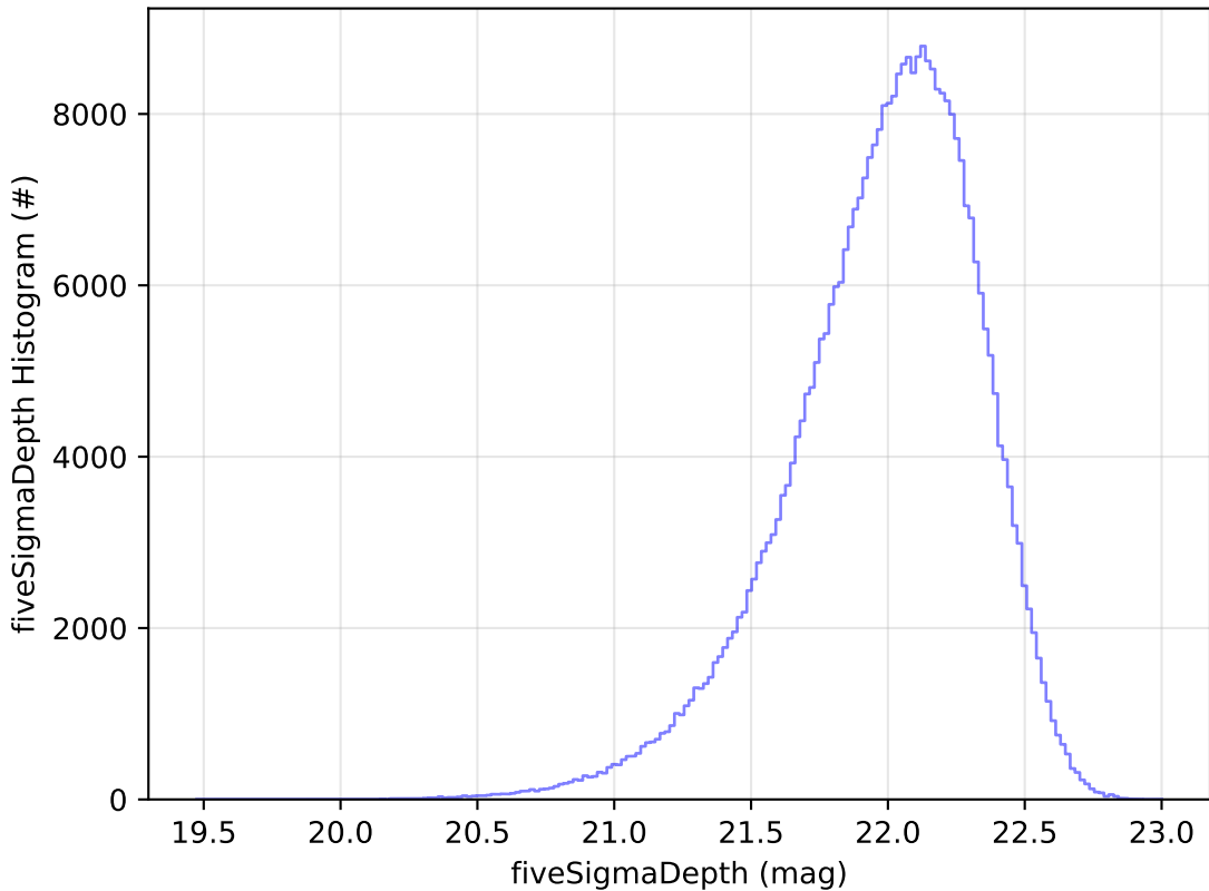
too_elab_2yr_r32_d2_ugrizy_v3.4_10yrs y: fiveSigmaDepth Histogram
