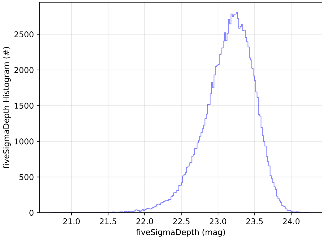
too_elab_2yr_r32_d2_ugrizy_v3.4_10yrs u: fiveSigmaDepth Histogram
