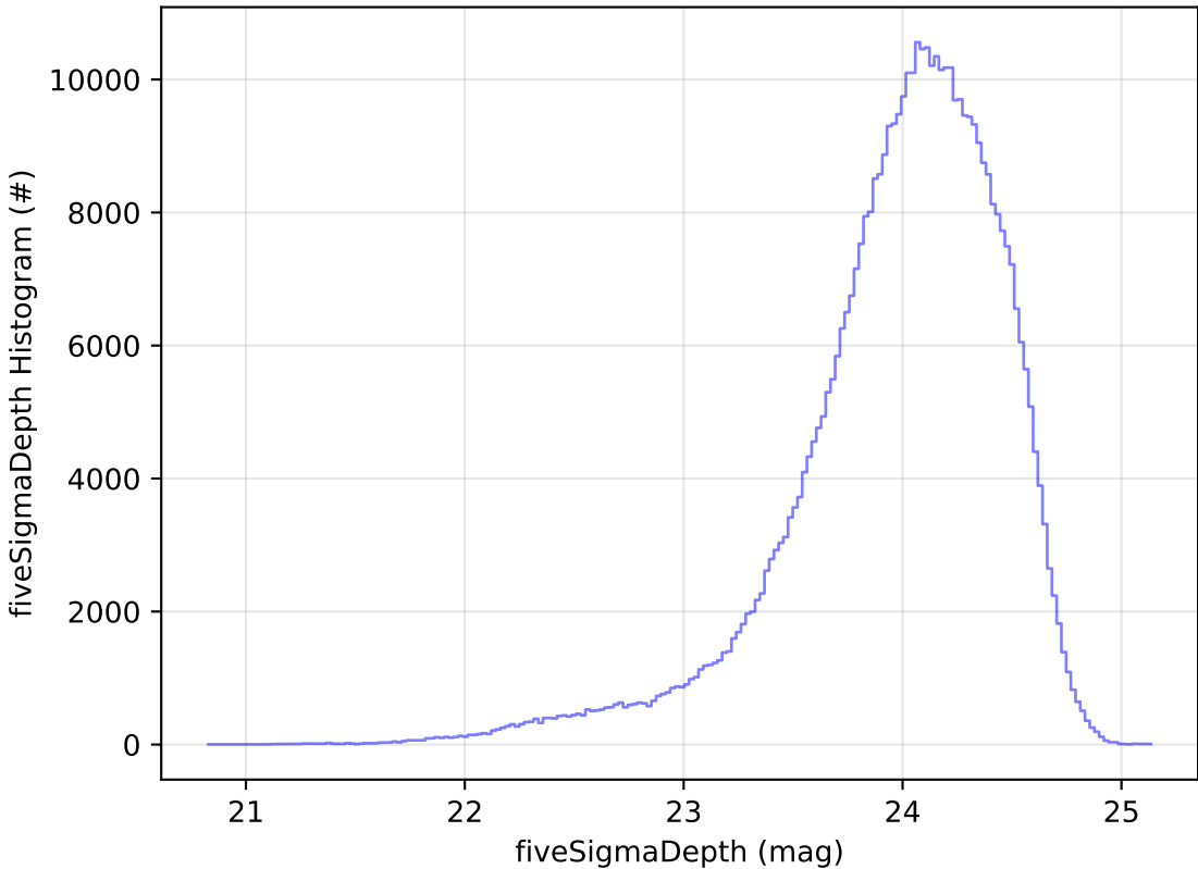
too_elab_2yr_r32_d2_ugrizy_v3.4_10yrs r: fiveSigmaDepth Histogram
