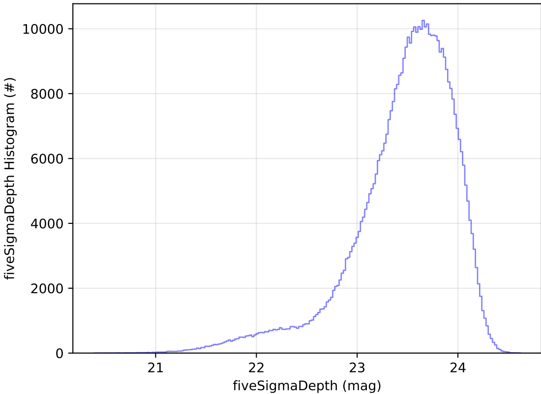
too_elab_2yr_r32_d2_ugrizy_v3.4_10yrs i: fiveSigmaDepth Histogram
