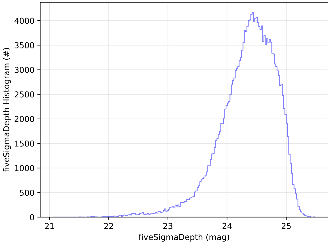
too_elab_2yr_r32_d2_ugrizy_v3.4_10yrs g: fiveSigmaDepth Histogram
