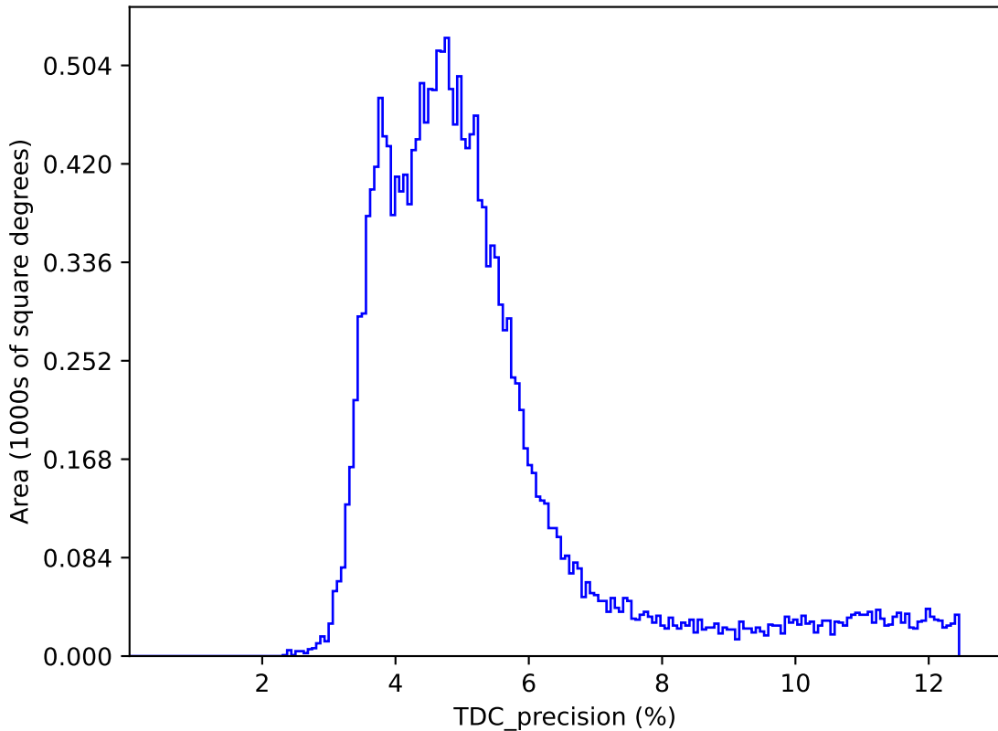
too_elab_2yr_r32_d2_ugrizy_v3.4_10yrs : TDC_precision
