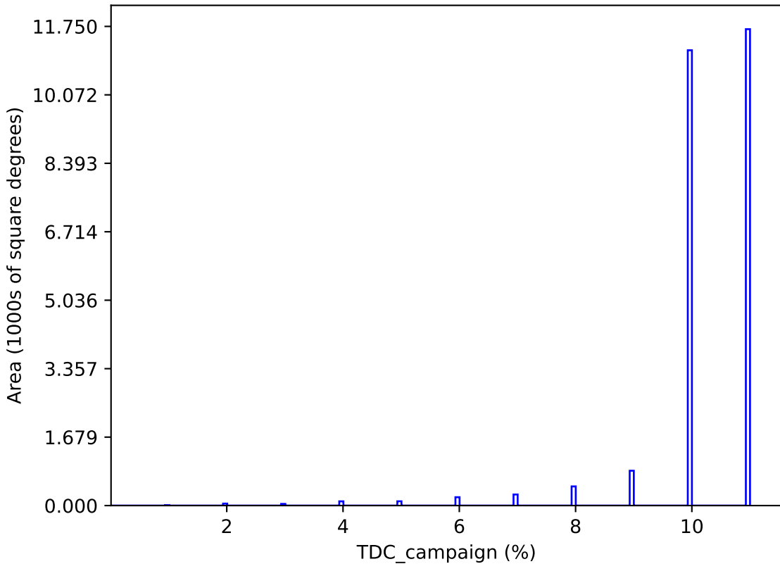
too_elab_2yr_r32_d2_ugrizy_v3.4_10yrs : TDC_campaign
