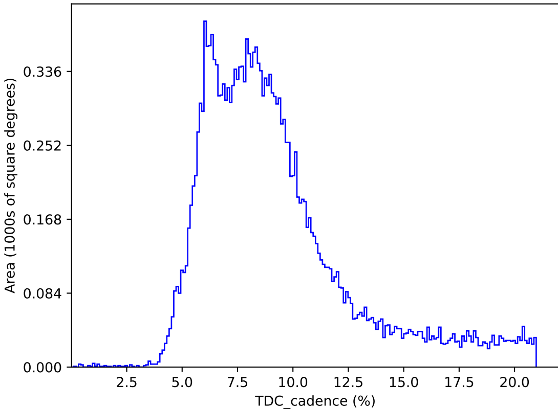
too_elab_2yr_r32_d2_ugrizy_v3.4_10yrs : TDC_cadence
