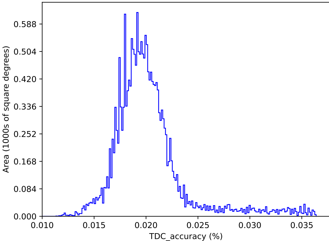
too_elab_2yr_r32_d2_ugrizy_v3.4_10yrs : TDC_accuracy
