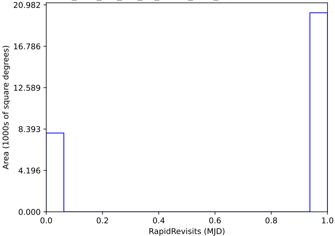
too_elab_2yr_r32_d2_ugrizy_v3.4_10yrs : RapidRevisits
