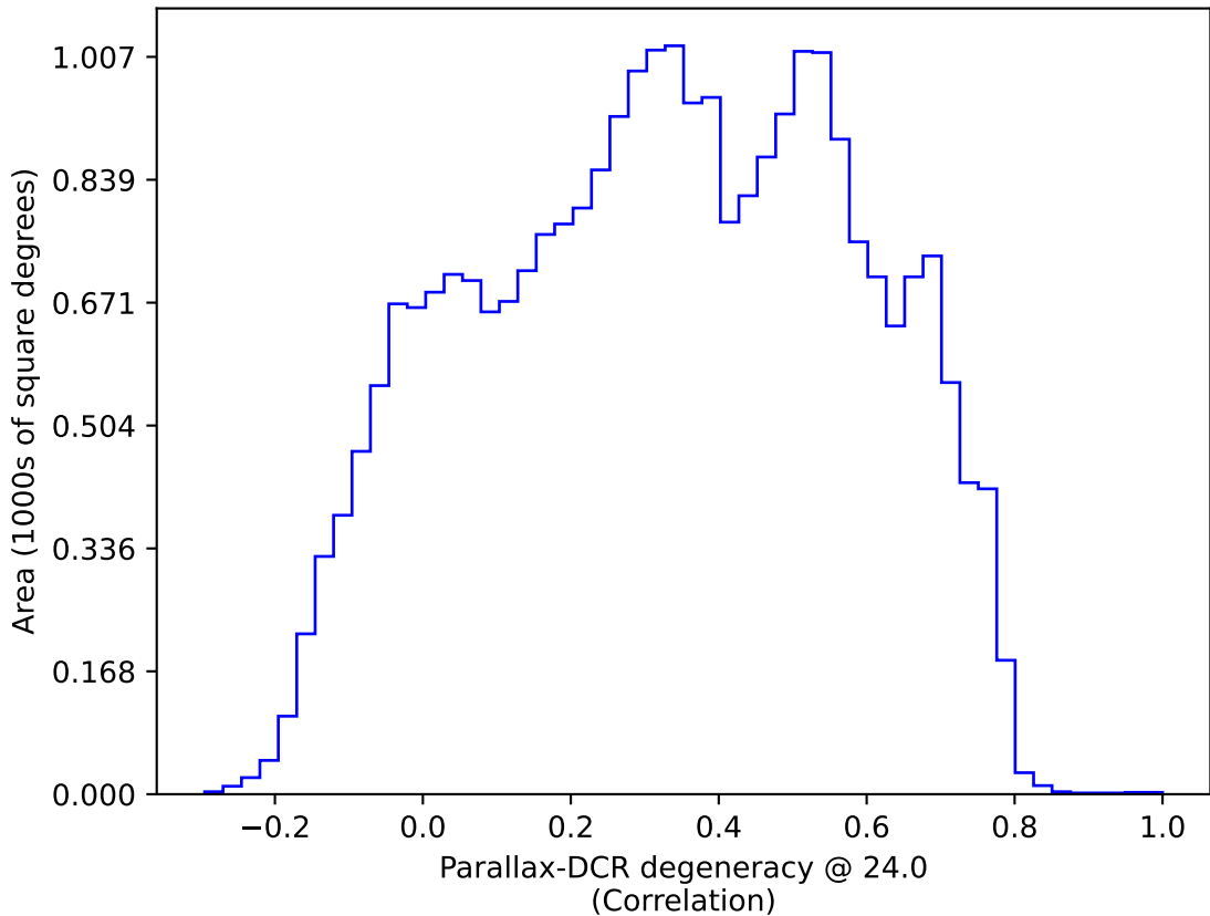
too_elab_2yr_r32_d2_ugrizy_v3.4_10yrs : Parallax-DCR degeneracy @ 24.0
