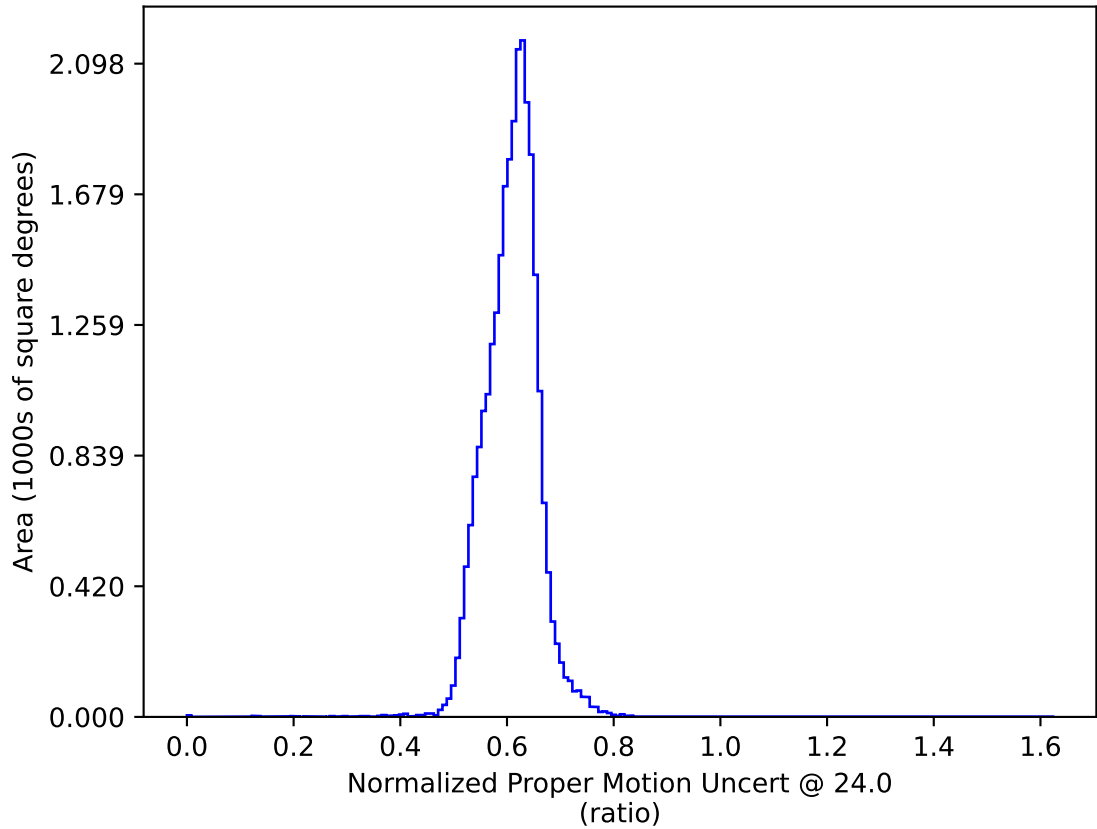
too_elab_2yr_r32_d2_ugrizy_v3.4_10yrs : Normalized Proper Motion Uncert @ 24.0
