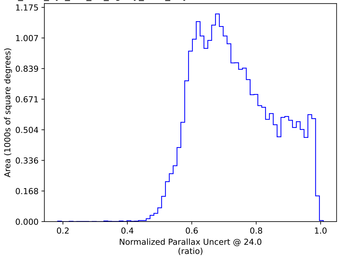
too_elab_2yr_r32_d2_ugrizy_v3.4_10yrs : Normalized Parallax Uncert @ 24.0
