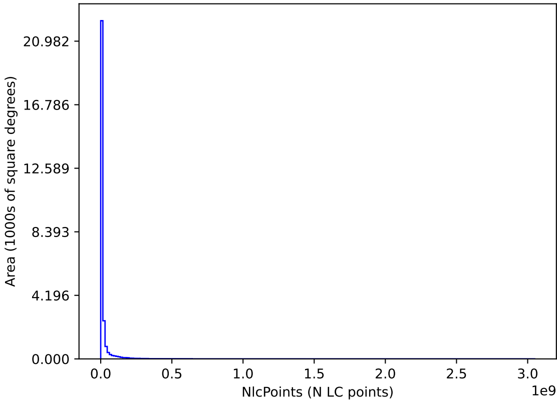
too_elab_2yr_r32_d2_ugrizy_v3.4_10yrs : NlcPoints
