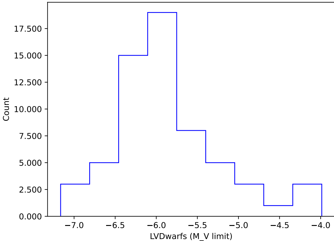
too_elab_2yr_r32_d2_ugrizy_v3.4_10yrs gi: LVDwarfs
