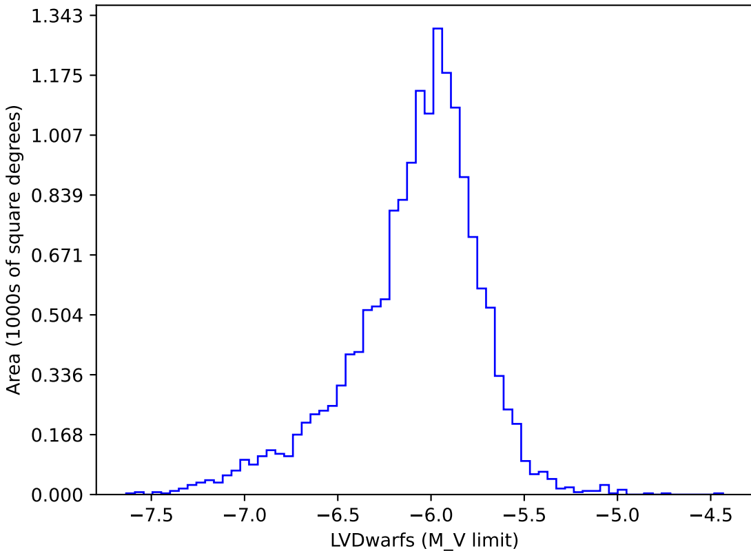
too_elab_2yr_r32_d2_ugrizy_v3.4_10yrs gi: LVDwarfs
