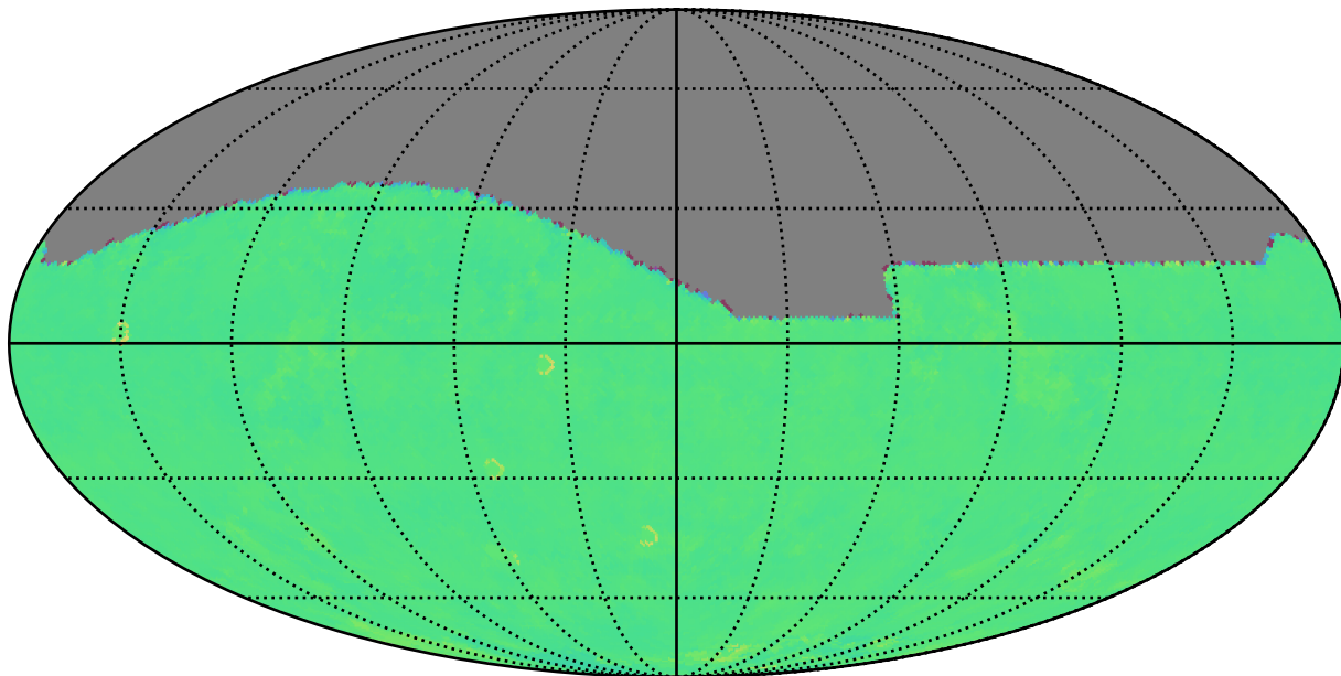
too_elab_2yr_r32_d2_ugrizy_v3.4_10yrs r: Kuiper rotTelPos
