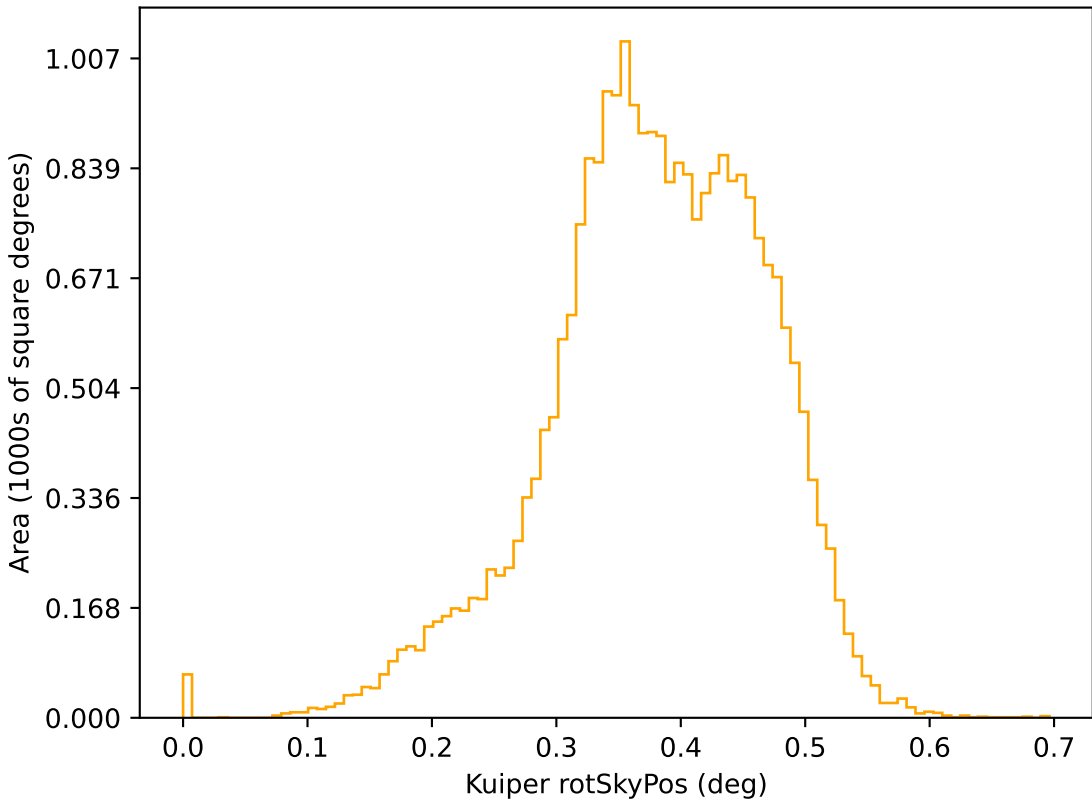
too_elab_2yr_r32_d2_ugrizy_v3.4_10yrs r: Kuiper rotSkyPos
