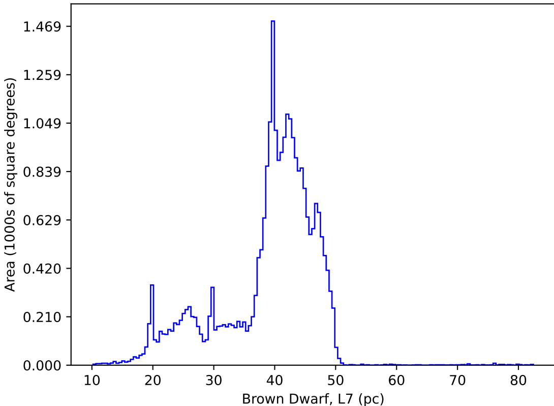
too_elab_2yr_r32_d2_ugrizy_v3.4_10yrs : Brown Dwarf, L7
