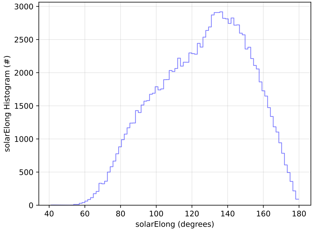
too_elab_2yr_r32_d2_ugrizy_v3.4_10yrs WFD u band: solarElong Histogram
