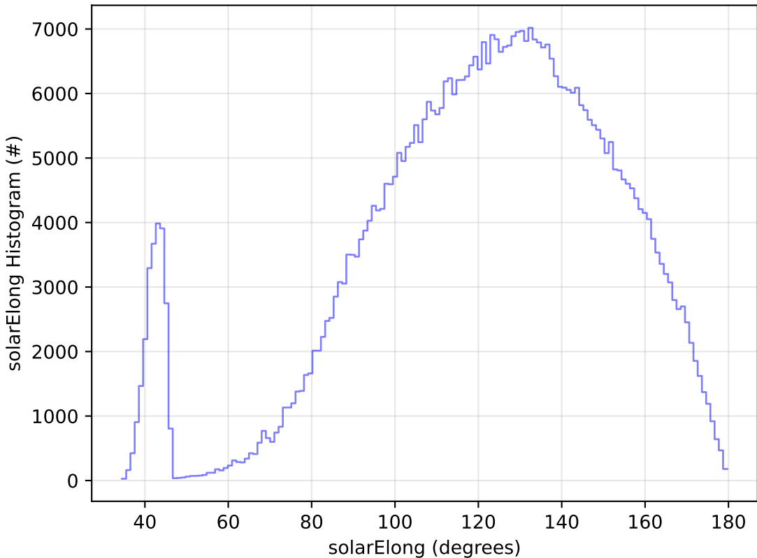
too_elab_2yr_r32_d2_ugrizy_v3.4_10yrs WFD i band: solarElong Histogram
