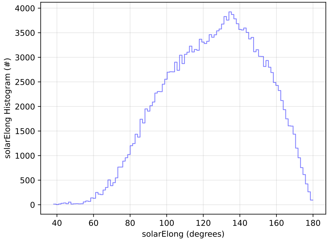
too_elab_2yr_r32_d2_ugrizy_v3.4_10yrs WFD g band: solarElong Histogram
