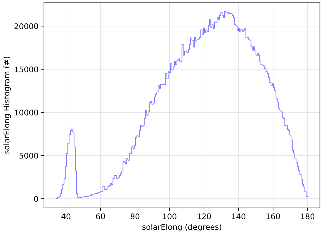
too_elab_2yr_r32_d2_ugrizy_v3.4_10yrs WFD all bands: solarElong Histogram
