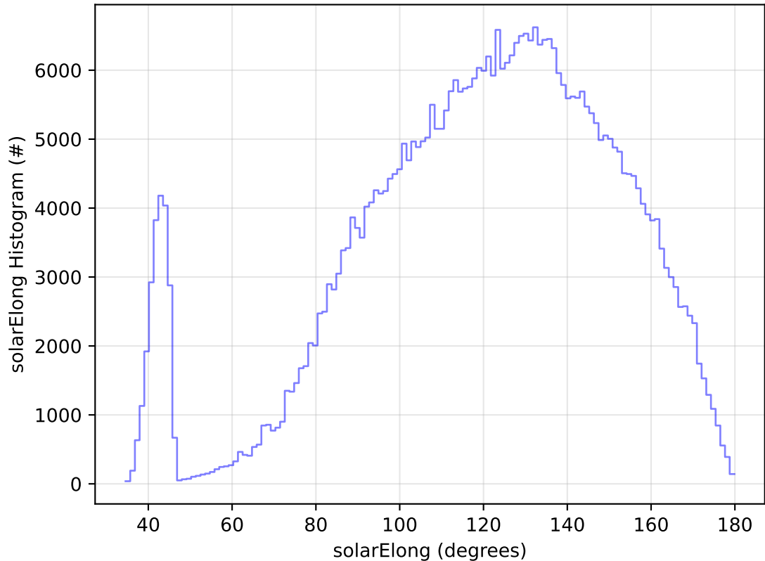
too_elab_2yr_r32_d2_ugrizy_v3.4_10yrs All sky z band: solarElong Histogram
