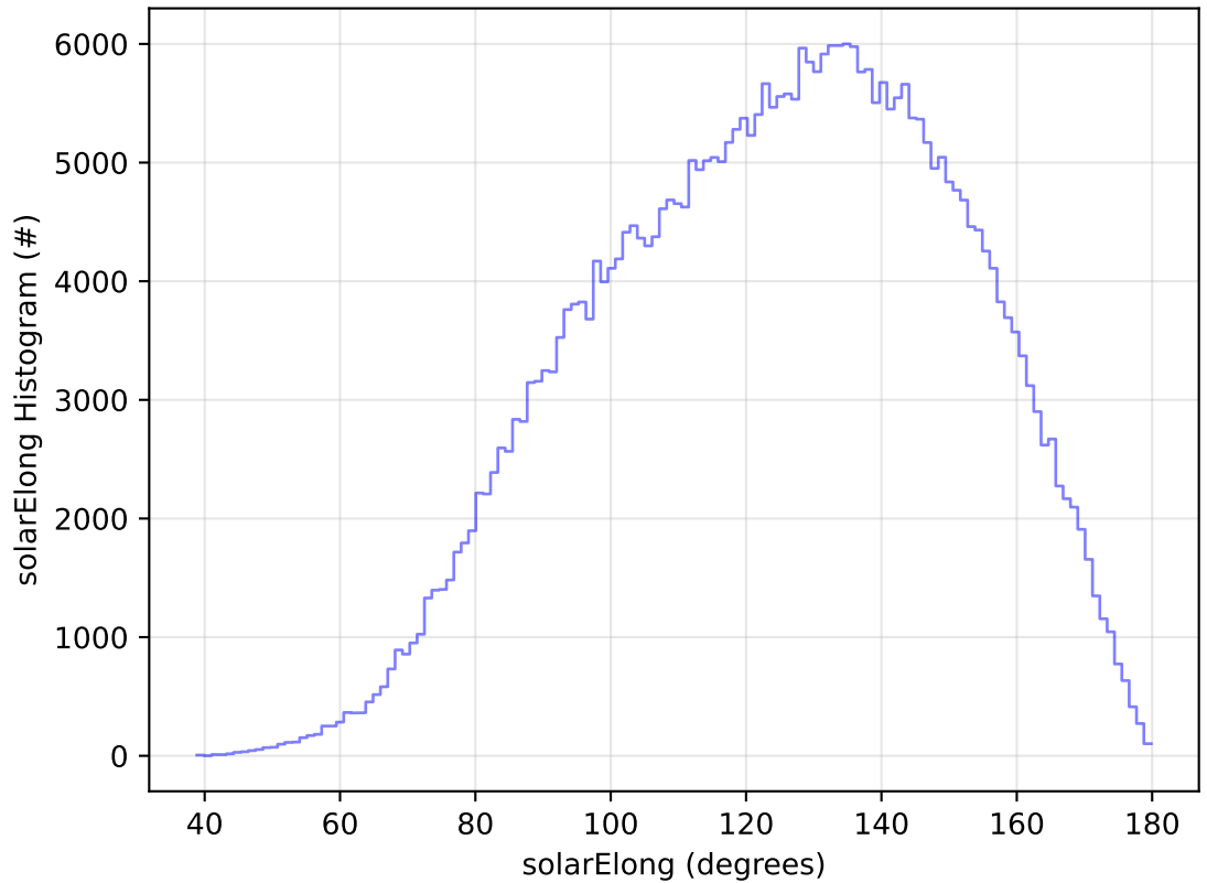
too_elab_2yr_r32_d2_ugrizy_v3.4_10yrs All sky y band: solarElong Histogram
