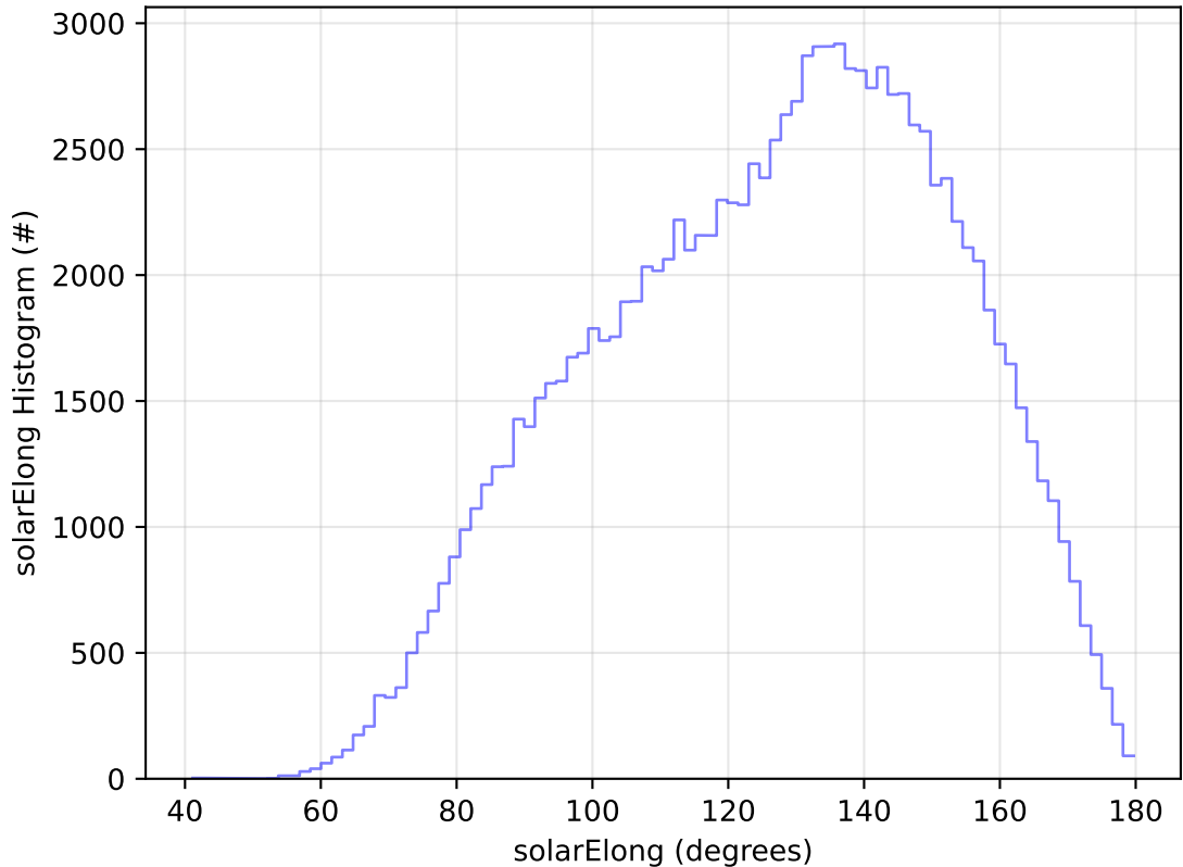
too_elab_2yr_r32_d2_ugrizy_v3.4_10yrs All sky u band: solarElong Histogram
