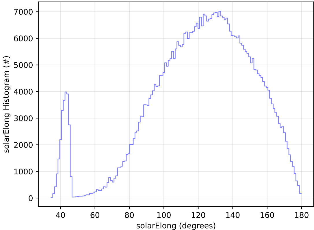
too_elab_2yr_r32_d2_ugrizy_v3.4_10yrs All sky i band: solarElong Histogram
