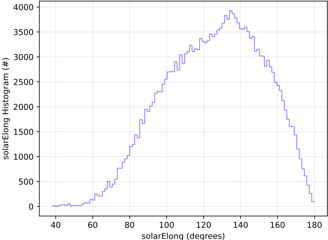
too_elab_2yr_r32_d2_ugrizy_v3.4_10yrs All sky g band: solarElong Histogram
