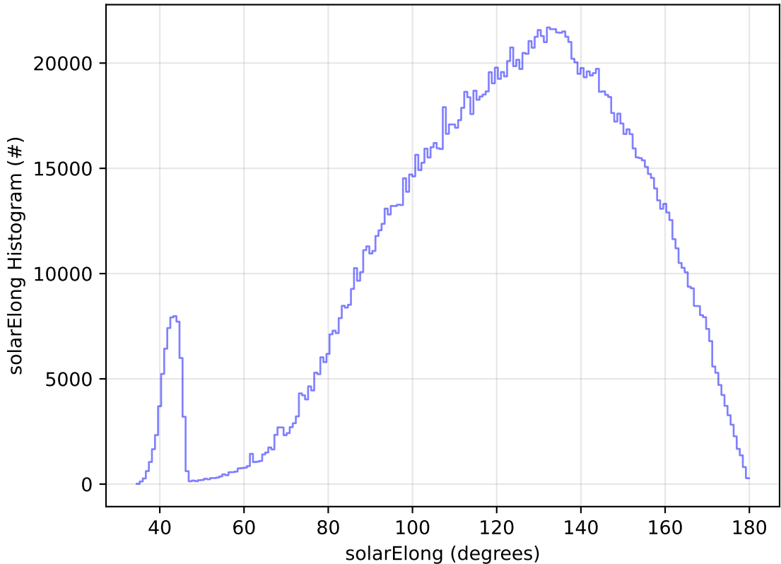
too_elab_2yr_r32_d2_ugrizy_v3.4_10yrs All sky all bands: solarElong Histogram
