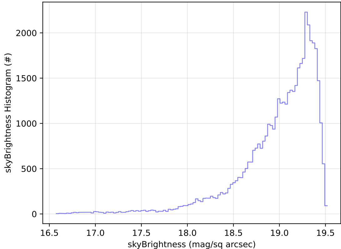
too_elab_2yr_r32_d2_ugrizy_v3.4_10yrs Yr 1 z band: skyBrightness Histogram
