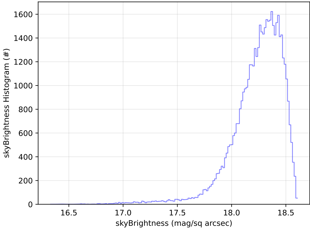
too_elab_2yr_r32_d2_ugrizy_v3.4_10yrs Yr 1 y band: skyBrightness Histogram
