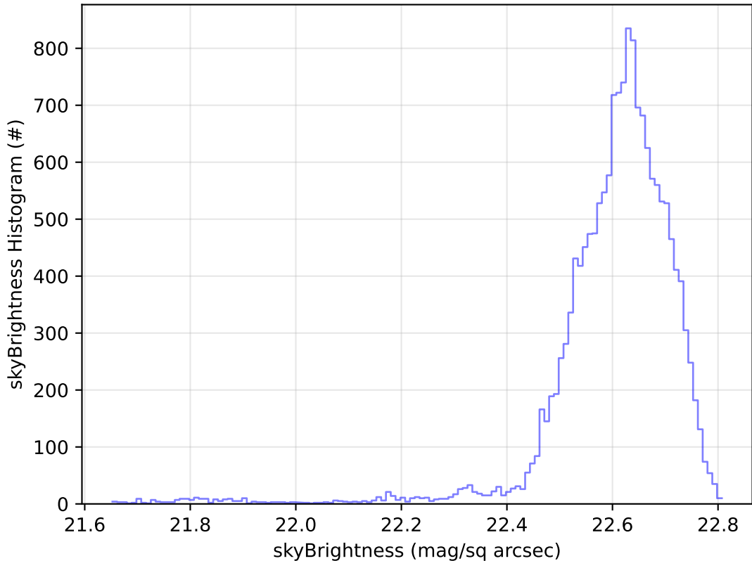
too_elab_2yr_r32_d2_ugrizy_v3.4_10yrs Yr 1 u band: skyBrightness Histogram
