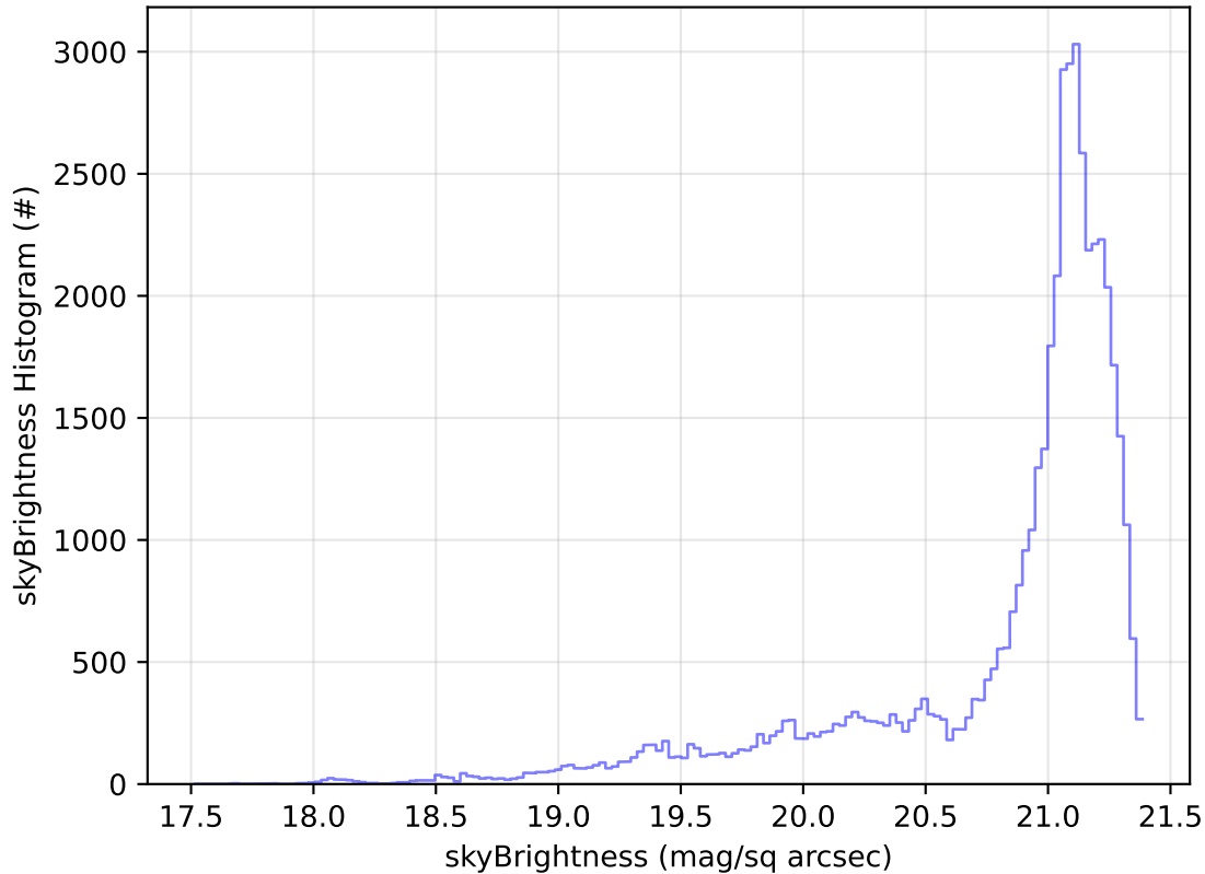
too_elab_2yr_r32_d2_ugrizy_v3.4_10yrs Yr 1 r band: skyBrightness Histogram
