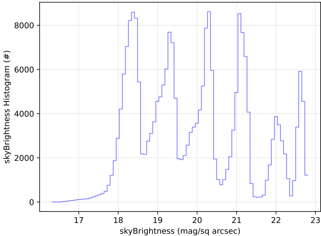
too_elab_2yr_r32_d2_ugrizy_v3.4_10yrs Yr 1 all bands: skyBrightness Histogram
