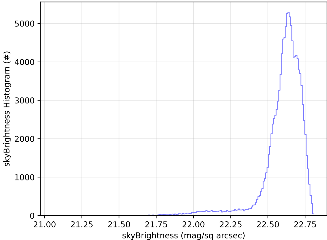
too_elab_2yr_r32_d2_ugrizy_v3.4_10yrs WFD u band: skyBrightness Histogram
