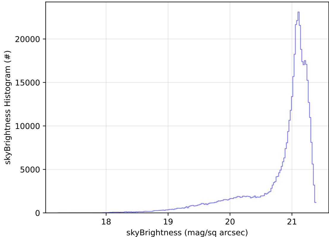
too_elab_2yr_r32_d2_ugrizy_v3.4_10yrs WFD r band: skyBrightness Histogram
