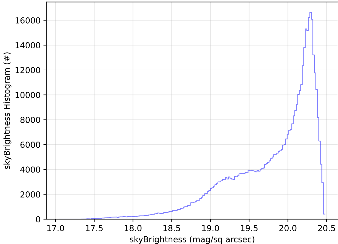
too_elab_2yr_r32_d2_ugrizy_v3.4_10yrs WFD i band: skyBrightness Histogram
