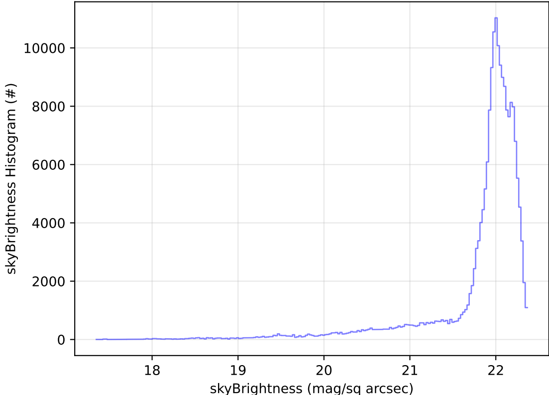
too_elab_2yr_r32_d2_ugrizy_v3.4_10yrs WFD g band: skyBrightness Histogram
