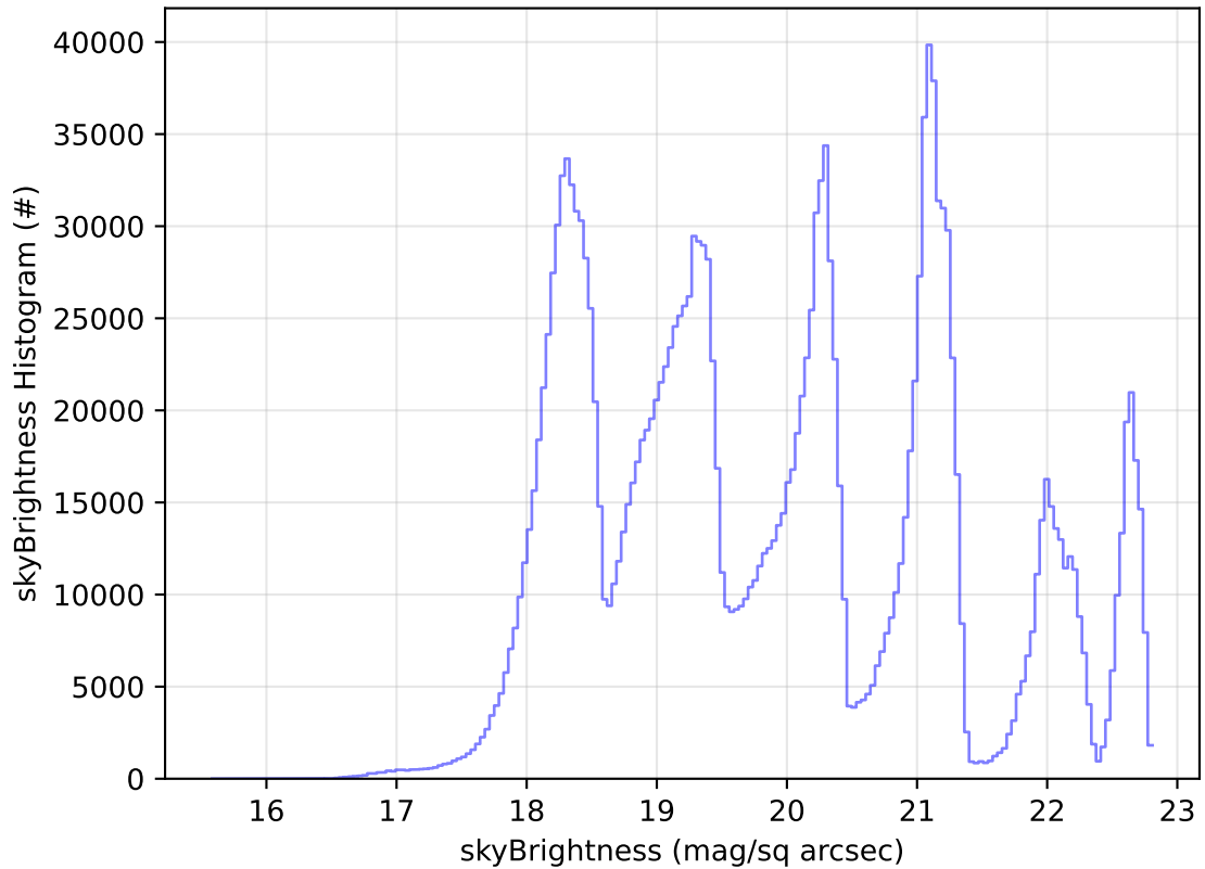
too_elab_2yr_r32_d2_ugrizy_v3.4_10yrs WFD all bands: skyBrightness Histogram
