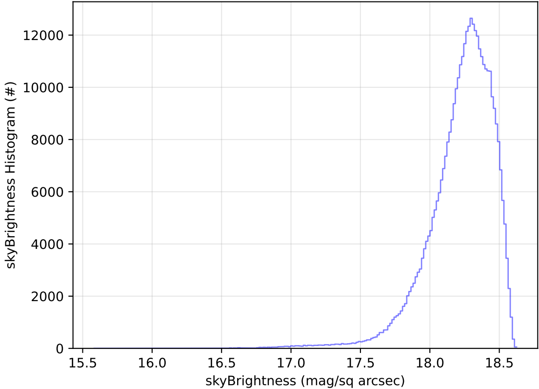
too_elab_2yr_r32_d2_ugrizy_v3.4_10yrs All sky y band: skyBrightness Histogram
