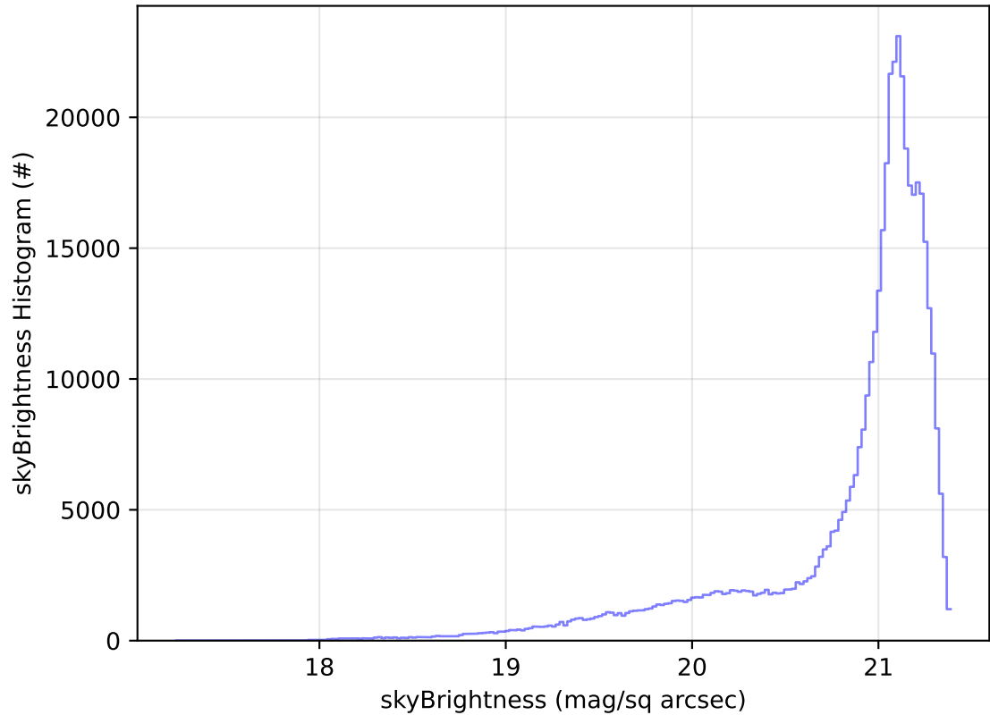
too_elab_2yr_r32_d2_ugrizy_v3.4_10yrs All sky r band: skyBrightness Histogram
