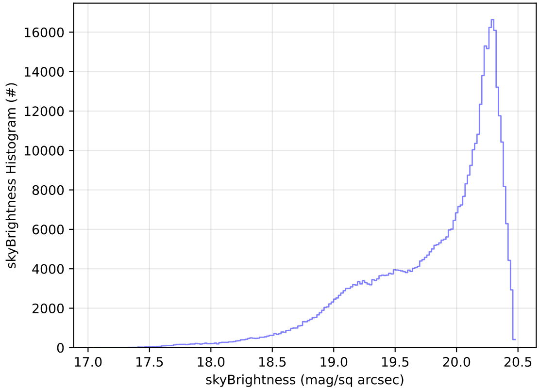
too_elab_2yr_r32_d2_ugrizy_v3.4_10yrs All sky i band: skyBrightness Histogram
