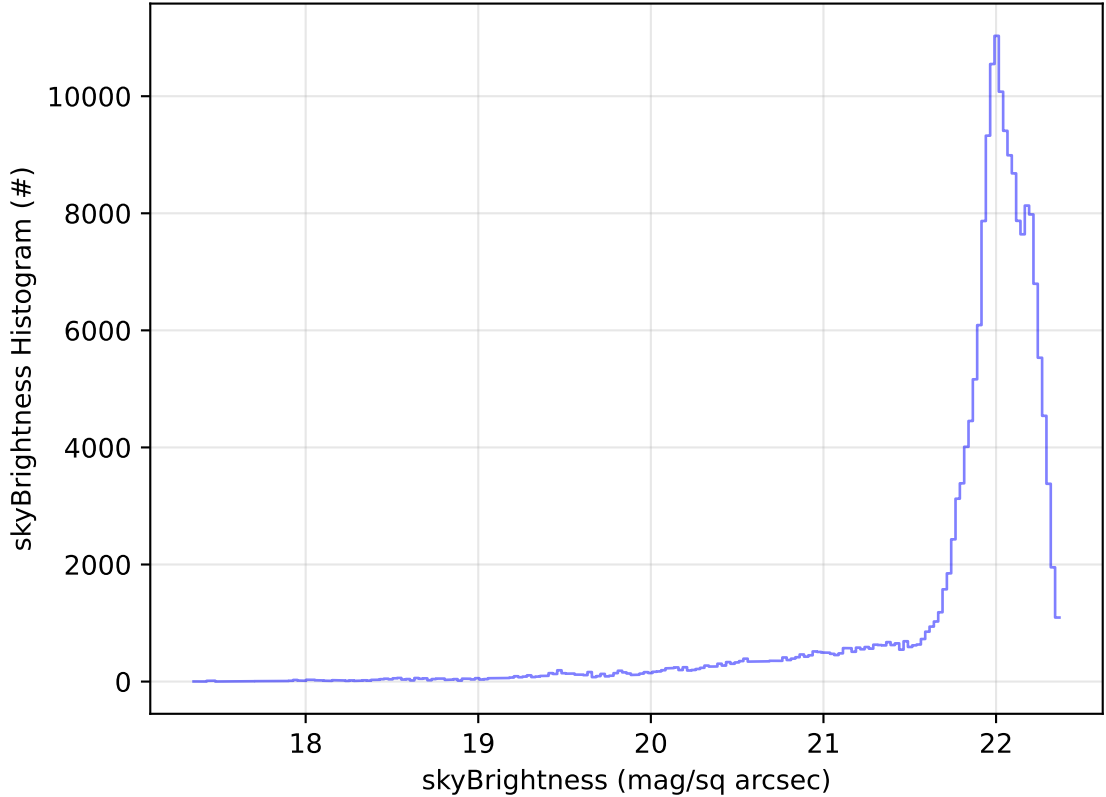
too_elab_2yr_r32_d2_ugrizy_v3.4_10yrs All sky g band: skyBrightness Histogram
